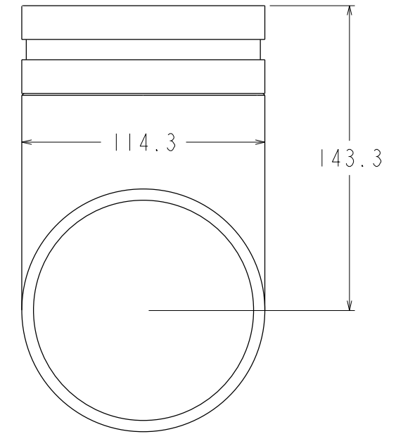
88PortBD-R2 4IN
