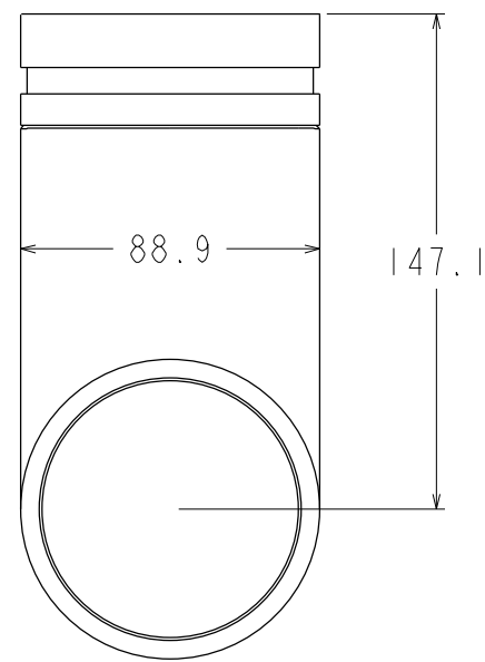
88PortBD-R3 3IN
